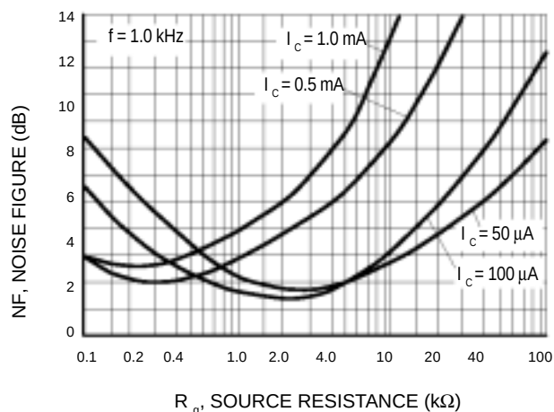
Figure 8. Noise Figure
