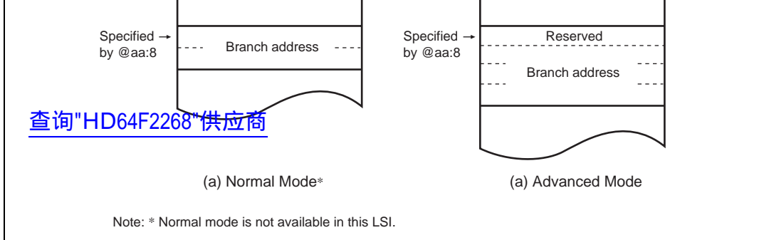
Figure 2.12 Branch Address Specification in Memory Indirect Mode
