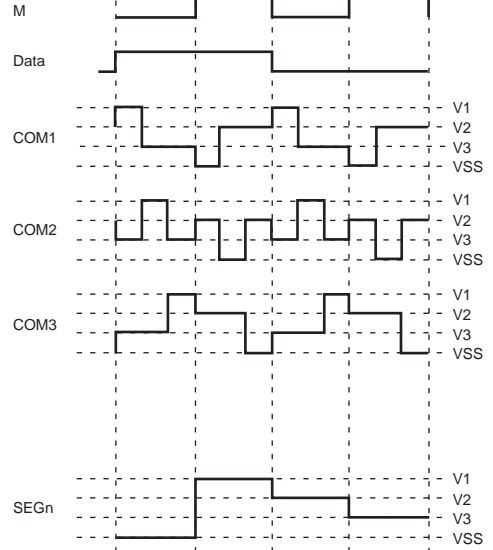
(b) Waveform with 1/3 duty
