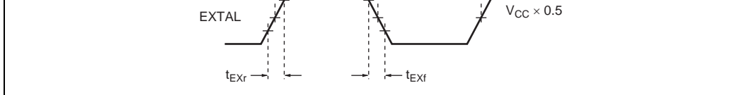
查询"HD64F2268"供应商 Figure 21.5 External Clock Input Timing
