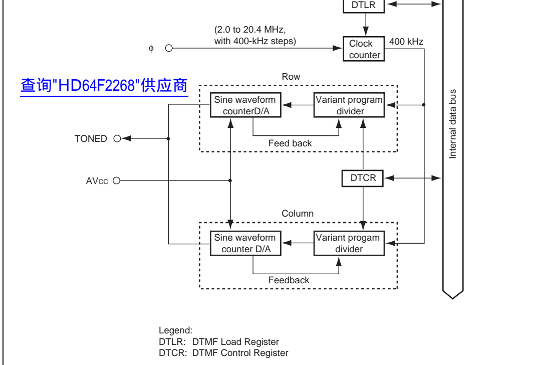
Figure 18.2 DTMF Generation Circuit Diagram
