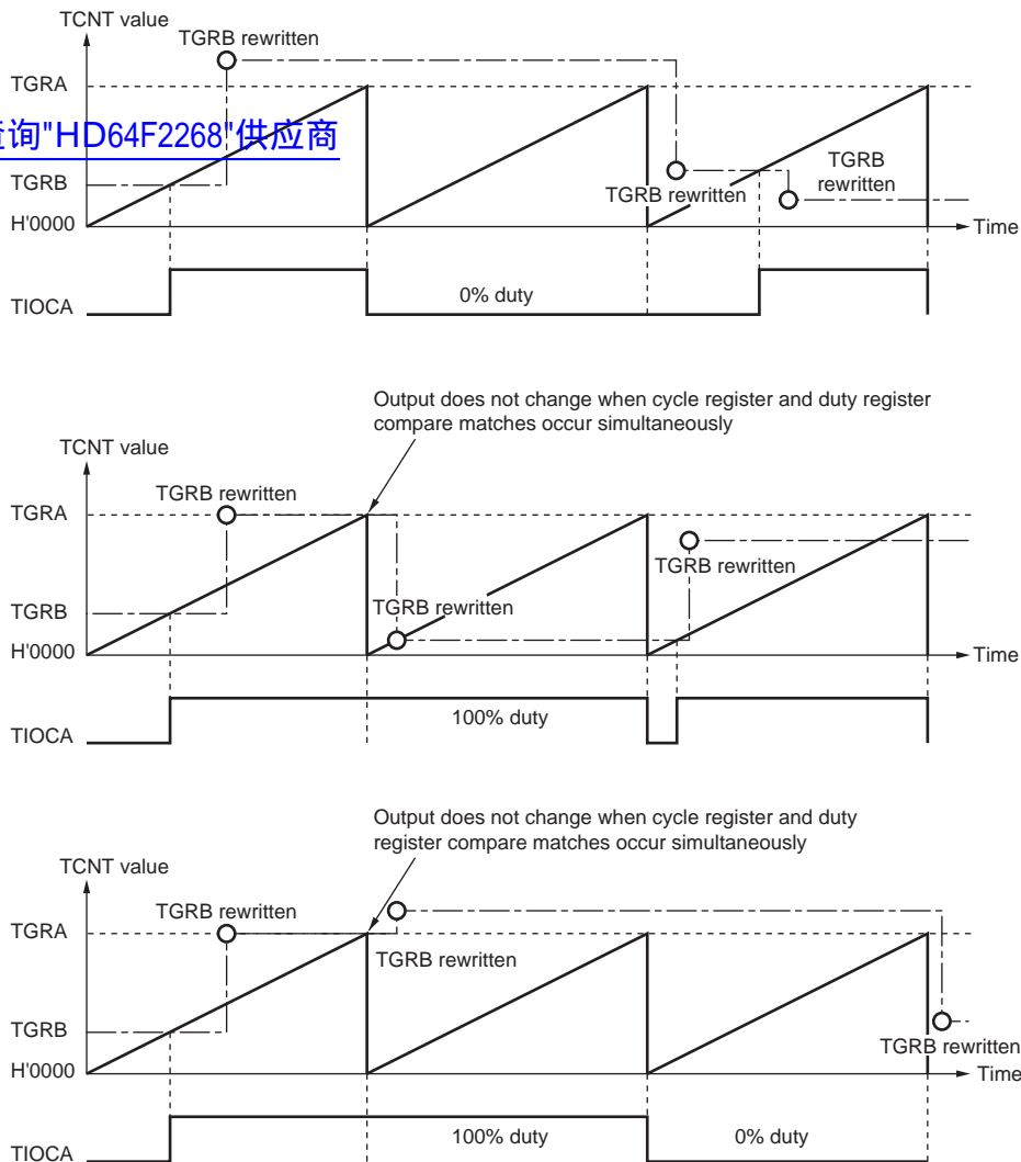
Figure 10.25 Example of PWM Mode Operation (3)
