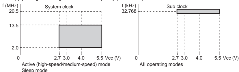
Figure 25.1 Power Supply Voltage and Operating Ranges (1)
