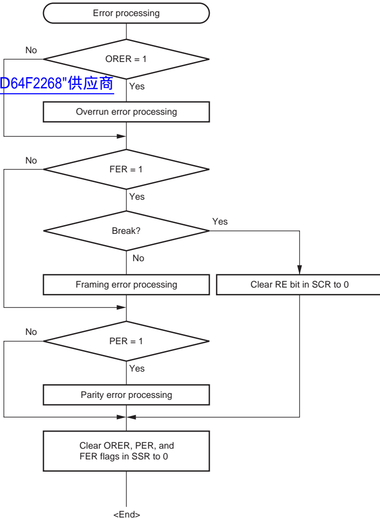
Figure 13.12 Sample Serial Reception Data Flowchart (2)
