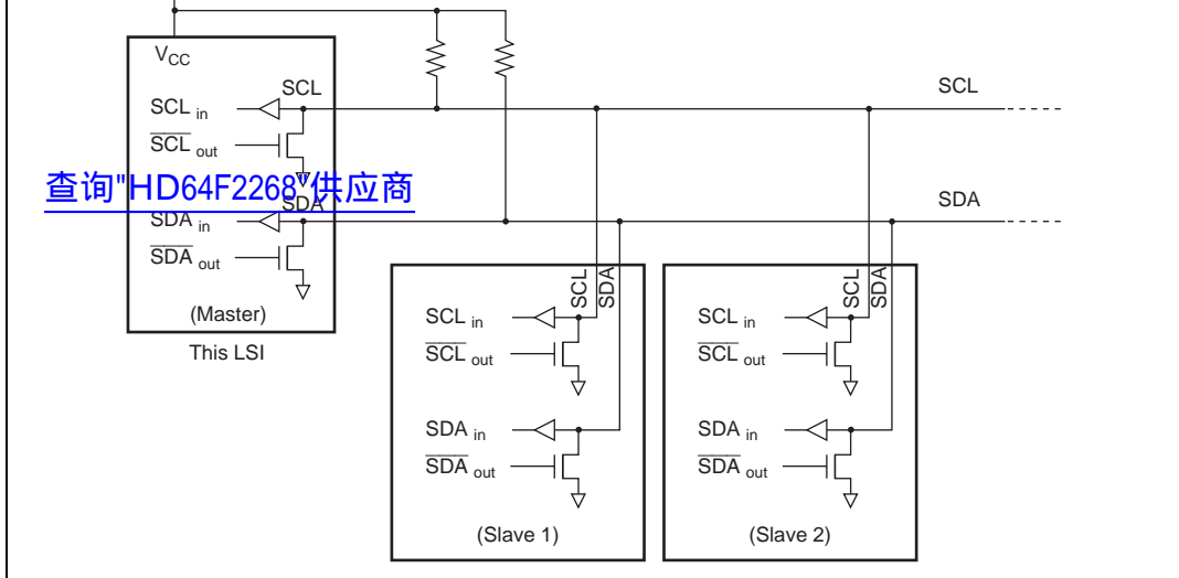
Figure 14.2 I²C Bus Interface Connections (Example: This LSI as Master)
