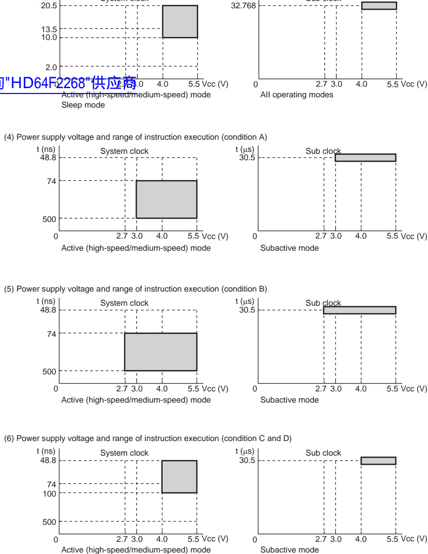
Figure 25.1 Power Supply Voltage and Operating Ranges (2)
