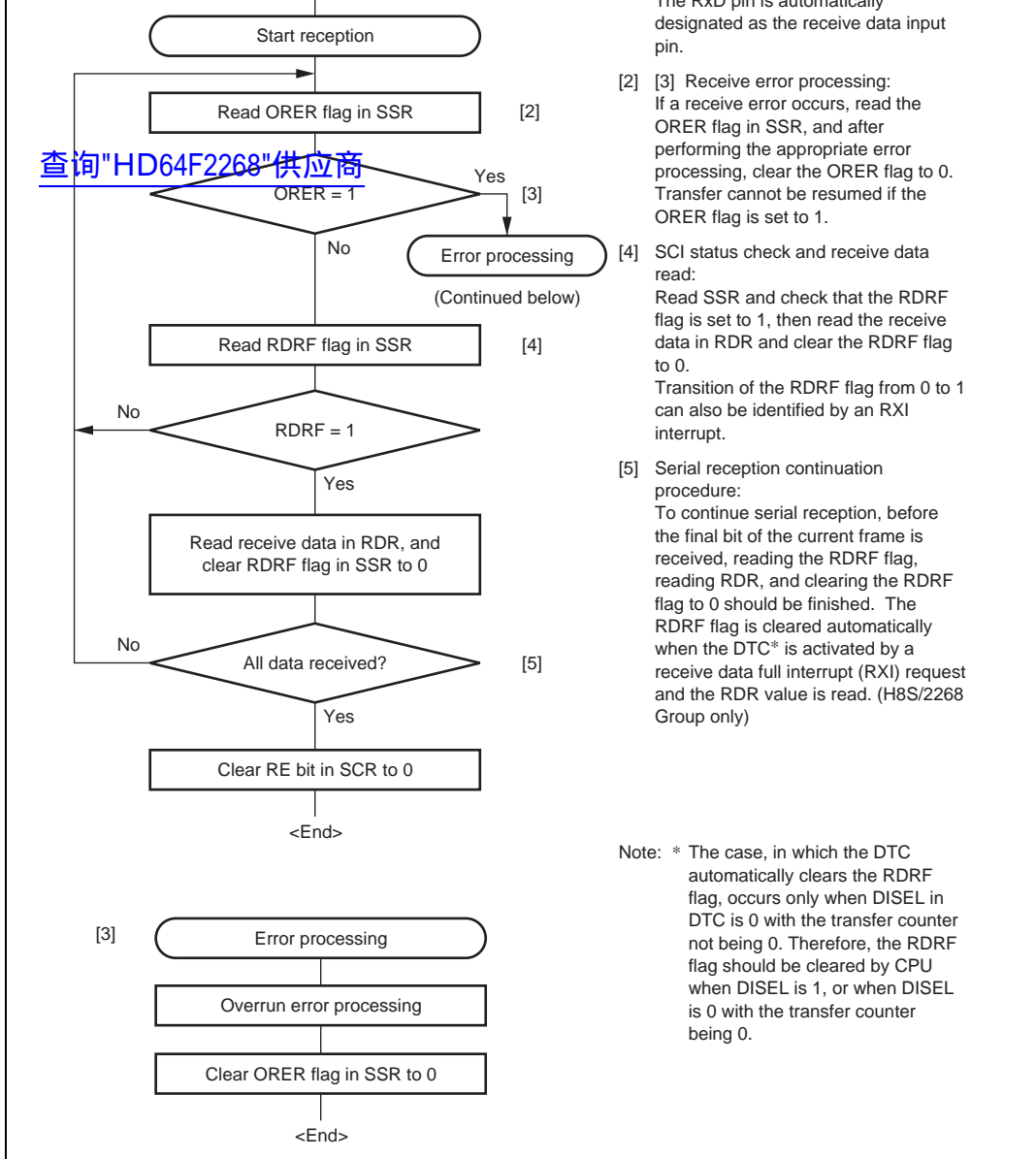
Figure 13.22 Sample Serial Reception Flowchart
