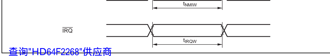
Figure 25.6 Interrupt Input Timing
