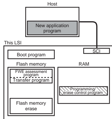
Figure 20.4 User Program Mode (Example)
