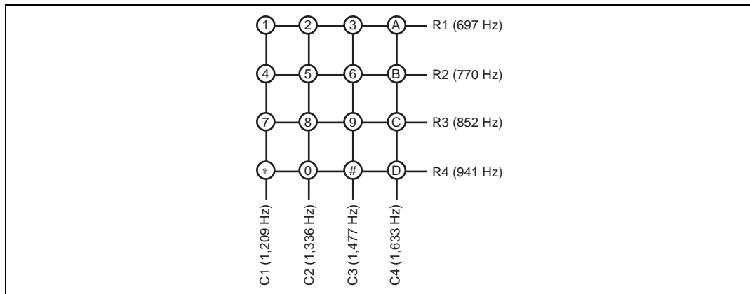
Figure 18.1 DTMF Frequencies
