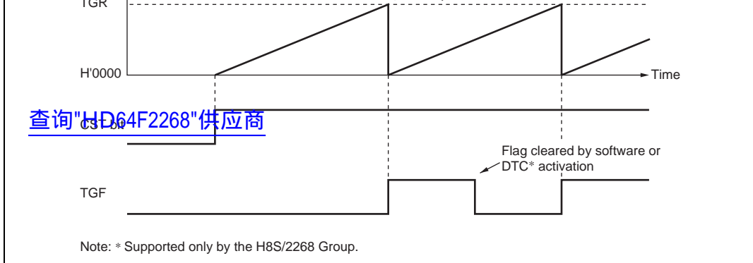
Figure 10.9 Periodic Counter Operation
