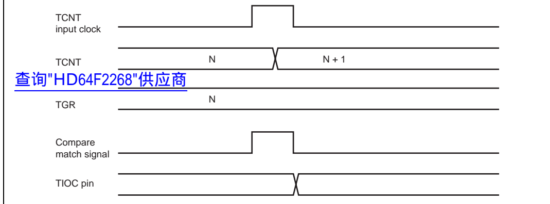
Figure 10.33 Output Compare Output Timing
