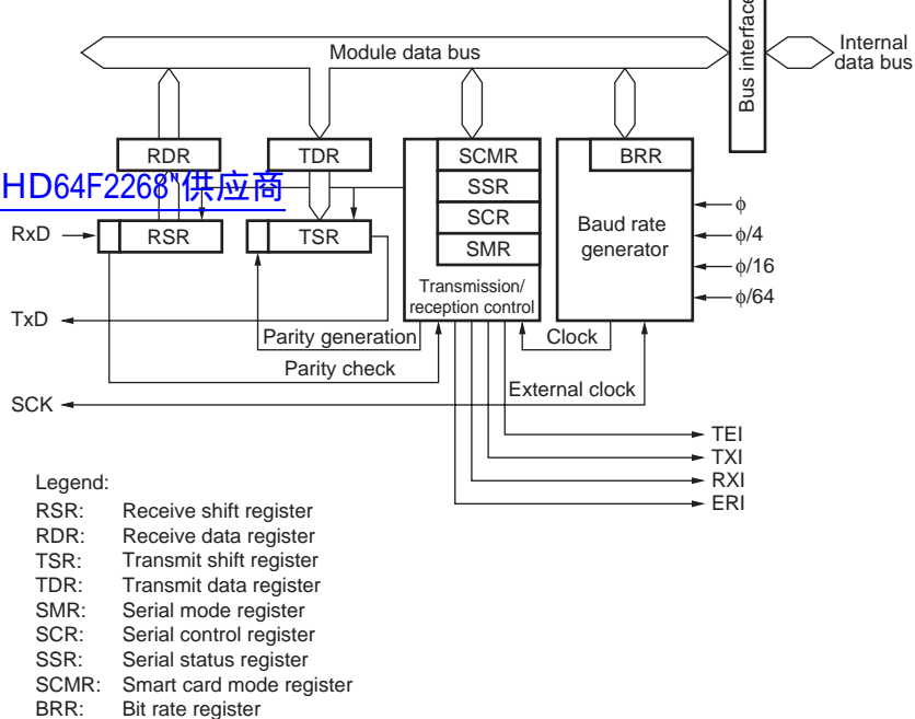
Figure 13.2 Block Diagram of SCI_1 or SCI_2
