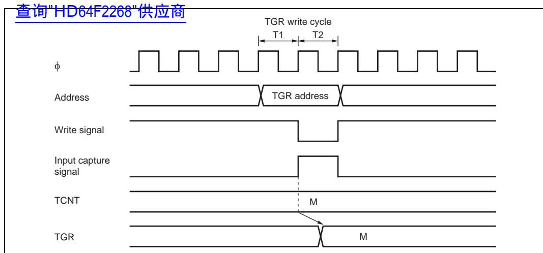
Figure 10.51 Contention between TGR Write and Input Capture
