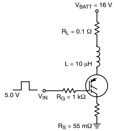
Figure 18. Circuit Configuration for Short Circuit Test #2
