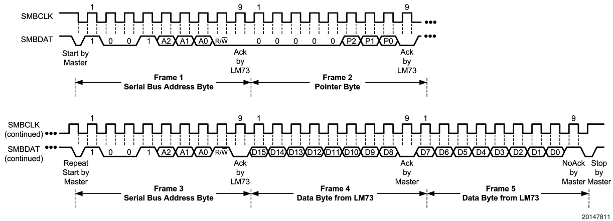
(b) Typical Pointer Set Followed by Immediate Read of a 2-Byte Register
