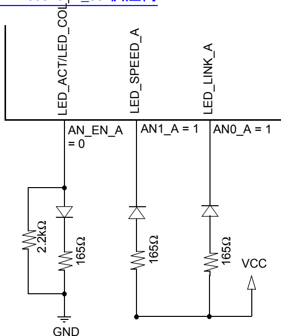
Figure 3. AN Strapping and LED Loading Example
