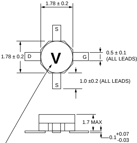
PACKAGE OUTLINE 84AS
