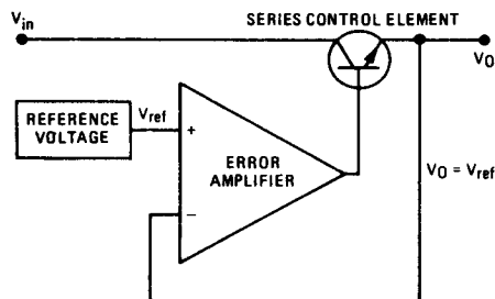
FIGURE 25 — SERIES VOLTAGE REGULATOR
