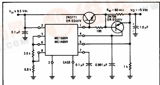
FIGURE 3 — TYPICAL NPN CURRENT BOOST CONNECTION ( V_0 = 5.0\text{ Vdc} , I_L = 10\text{ A dc (max)} )
