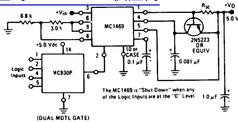
FIGURE 34 - ELECTRONIC SHUT-DOWN USING A MDTL GATE
