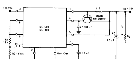
FIGURE 7 - LOAD REGULATION
