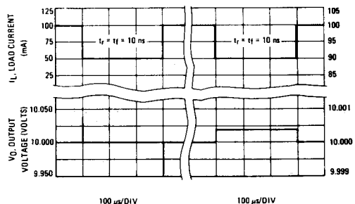
FIGURE 28B – LOAD TRANSIENT RESPONSE
