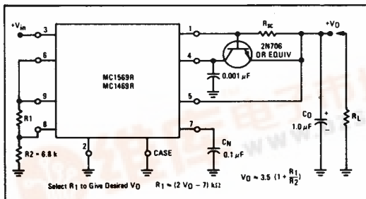
FIGURE 2 — TYPICAL CIRCUIT CONNECTION ( 3.5 \leq V_0 \leq 37\text{ Vdc} , 1 \leq I_L \leq 500\text{ mA} )
