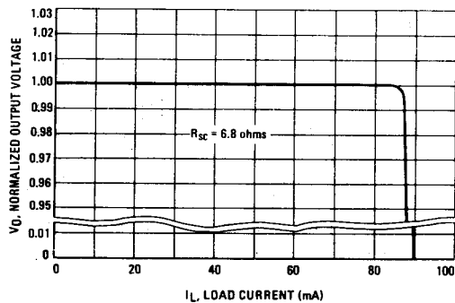
FIGURE 17 – CURRENT-LIMITING CHARACTERISTICS
