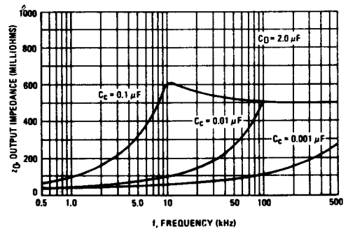
FIGURE 24 – FREQUENCY DEPENDENCE OF OUTPUT IMPEDANCE, C_O = 2.0 \mu\text{F}
