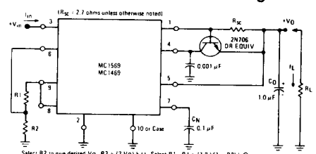
FIGURE 7 - LOAD REGULATION
