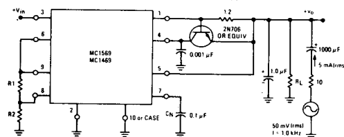
FIGURE 8 - OUTPUT IMPEDANCE
