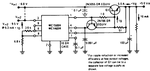
FIGURE 29B — 5-VOLT 5-AMPERE REGULATOR
