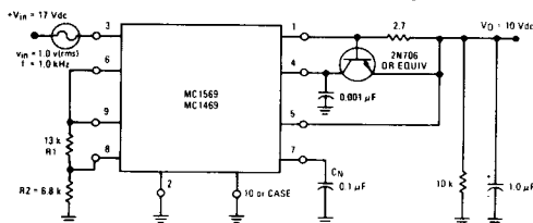
FIGURE 6 - INPUT REGULATION
