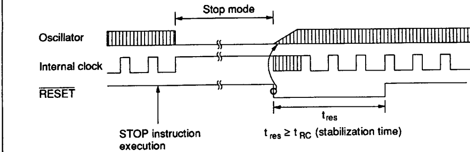
Figure 11 Timing of Stop Mode Cancellation
