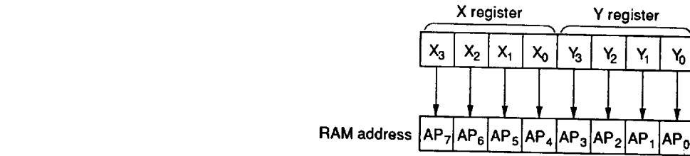
Register Indirect Addressing
