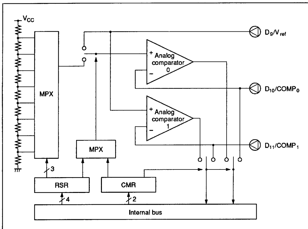
Figure 21 Comparator Block Diagram
