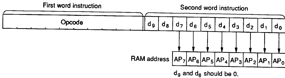
Direct Addressing
