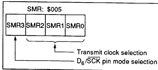
Transmit Clock
