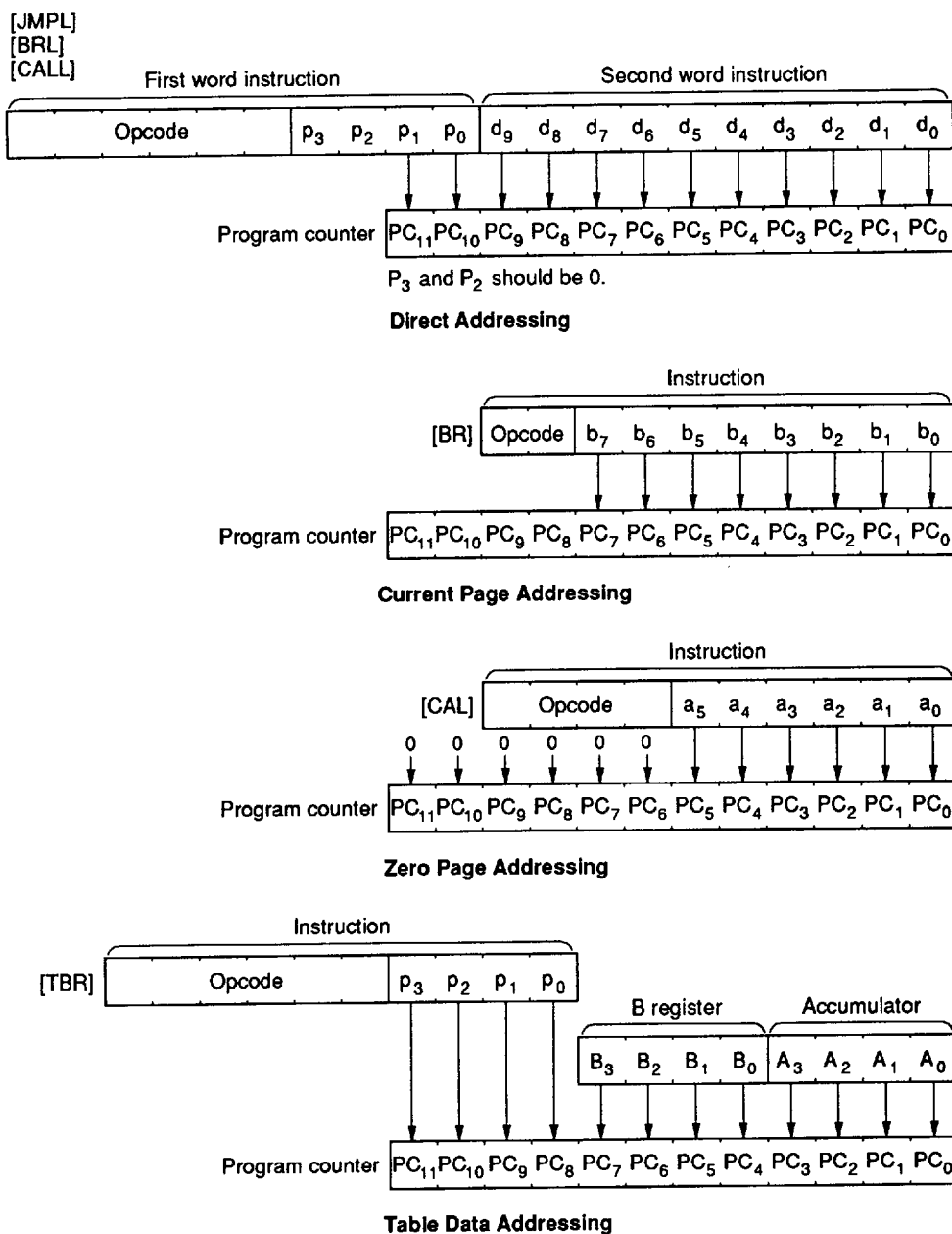
Figure 26 ROM Addressing Modes
