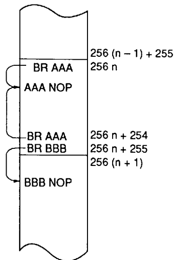
Figure 27 BR Instruction Branch Destination on a Page Boundary
