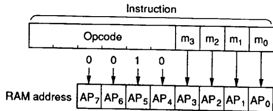
Memory Register Addressing
