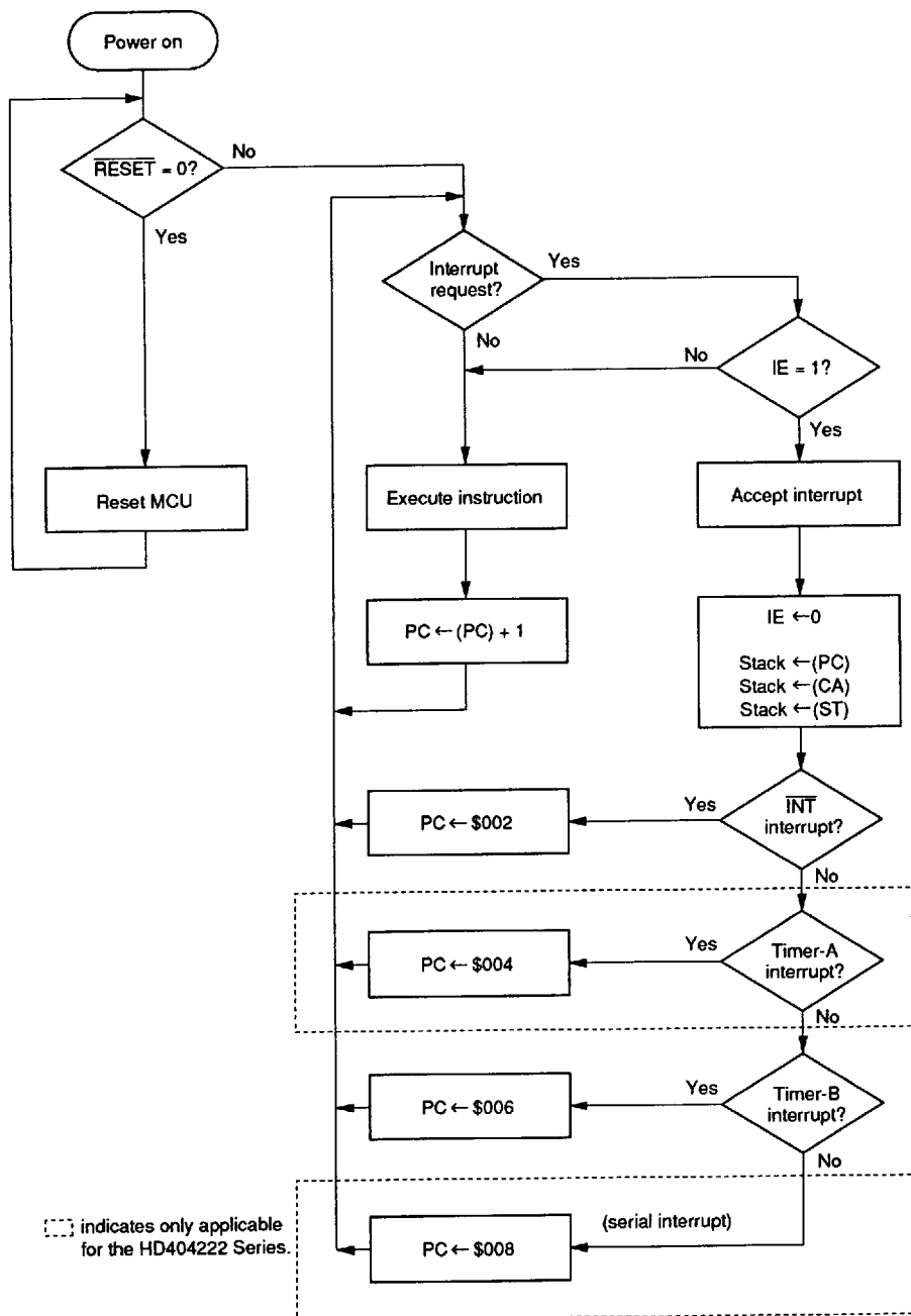
Figure 8 Interrupt Processing Flowchart
