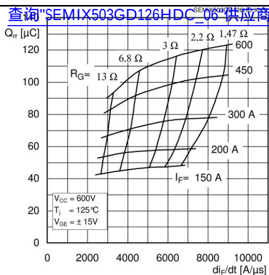
Fig. 13 Typ. CAL diode recovered charge
