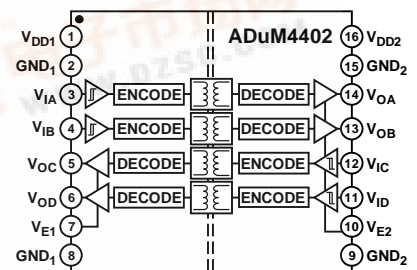
Figure 3. ADuM4402
