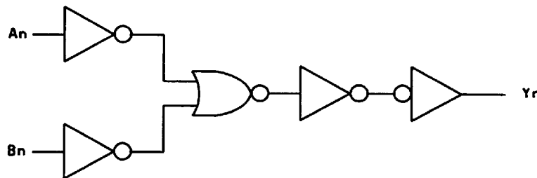
FIGURE 3. Logic diagram.
