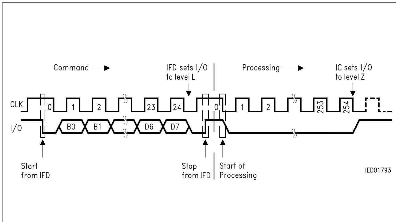
Figure 7 Erase and Write Main Memory
