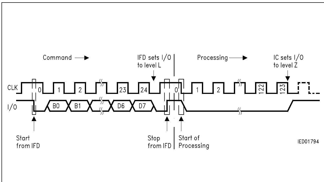
Figure 8 Erase or Write Main Memory
