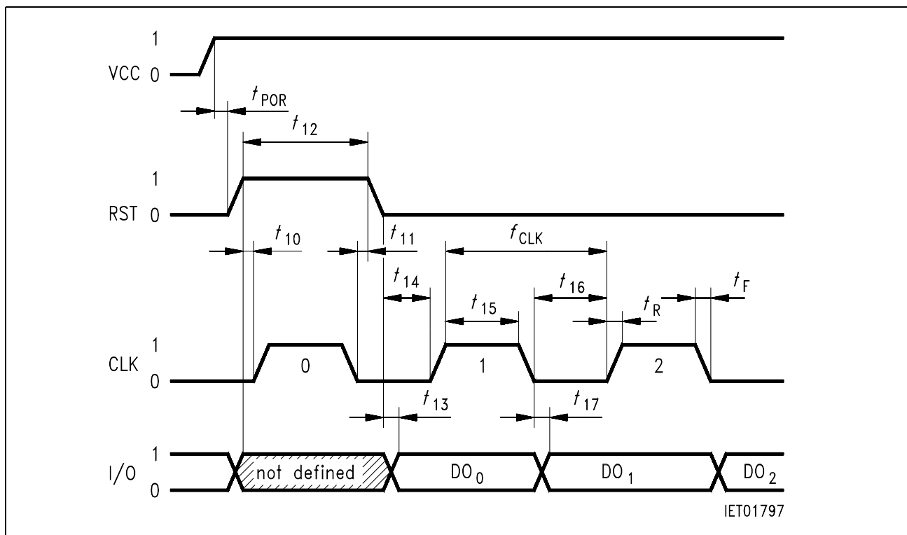
Figure 14 Reset and Answer-to-Reset
