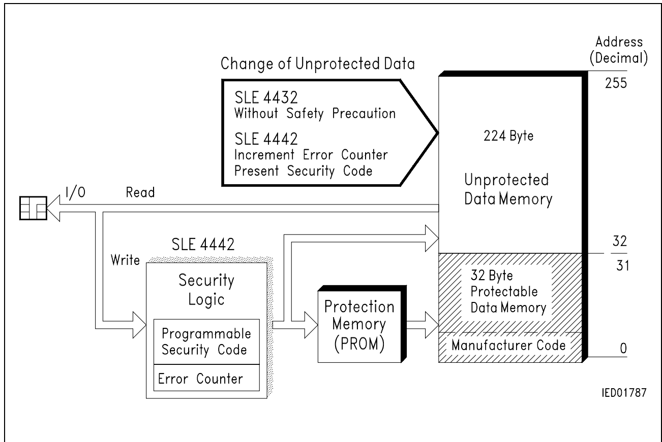
Figure 1 Memory Overview
