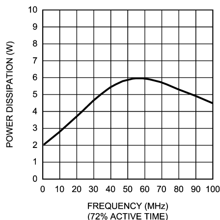
FIGURE 11. Power Dissipation vs Frequency
