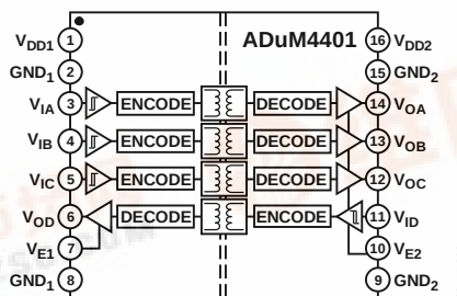
Figure 2. ADuM4401
