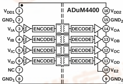
Figure 1. ADuM4400
