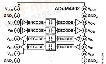
Figure 3. ADuM4402
