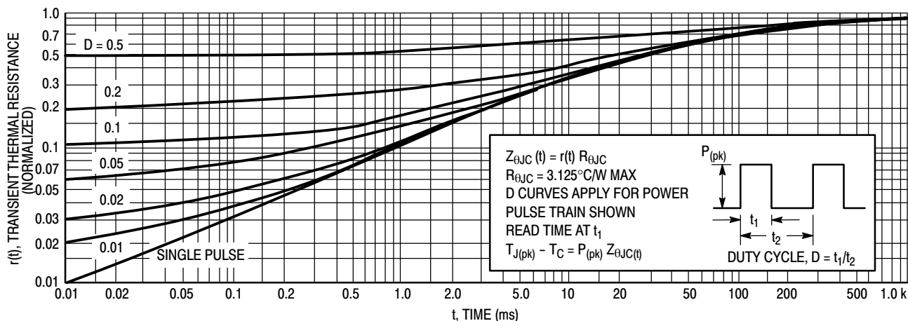
Figure 4. Thermal Response
