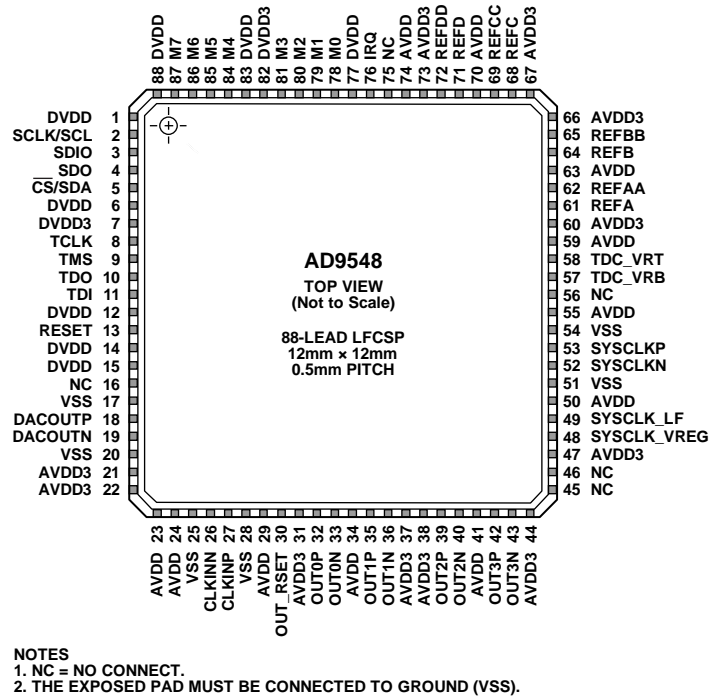
Figure 2. 88-Lead LFCSP Pin Configuration
