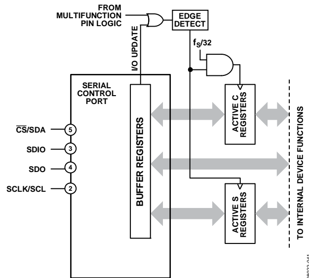
Figure 65. Buffered and Active Registers
