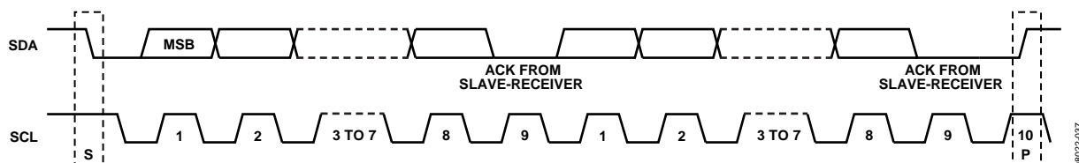
Figure 61. Acknowledge Bit
