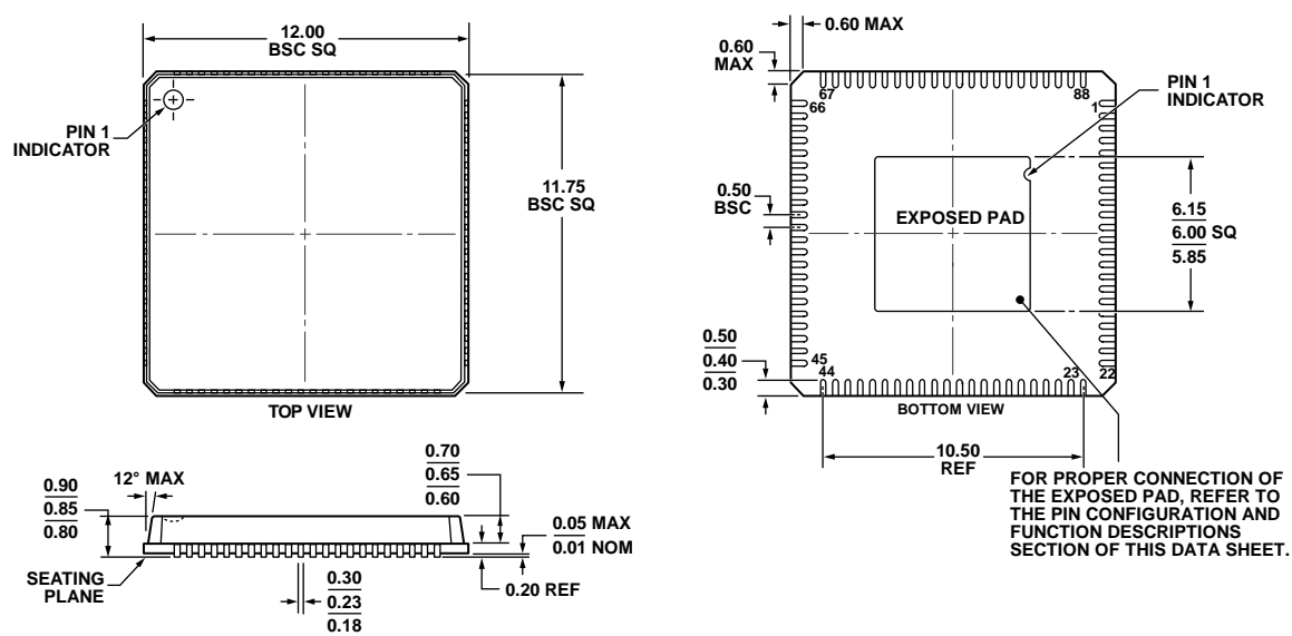
COMPLIANT TO JEDEC STANDARDS MO-220-VRRD. Figure 68. 88-Lead Lead Frame Chip Scale Package [LFCSP_VQ] 12 mm × 12 mm Body, Very Thin Quad (CP-88-2) Dimensions shown in millimeters
