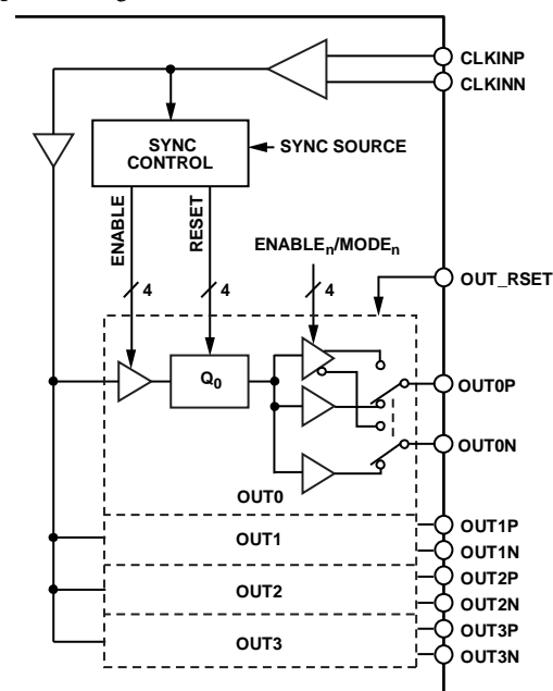
Figure 47. Clock Distribution
