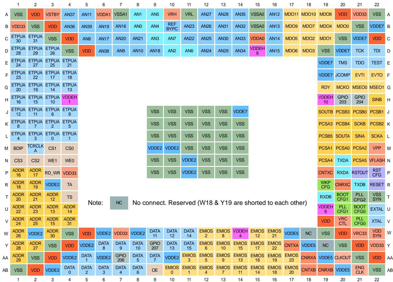
Figure 28. MPC5565 324 Package
