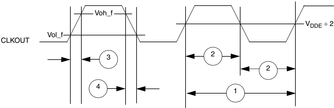
Figure 12. CLKOUT Timing
