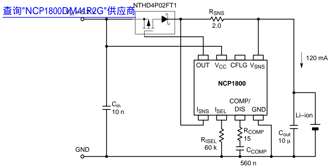
Figure 17. Typical Application Circuit for Lower Capacity Batteries (120 mAh shown here)
