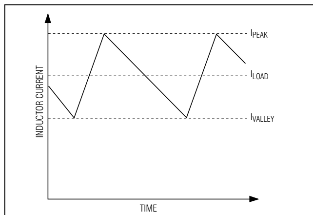
Figure 5. Inductor-Current Waveform
