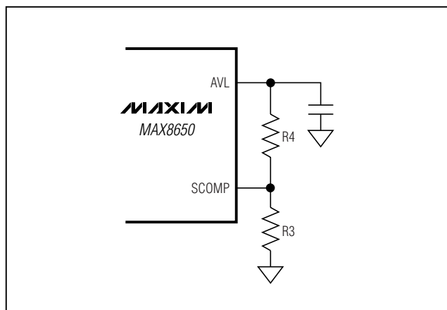
Figure 6. Resistor-Divider for Setting the Slope Compensation
