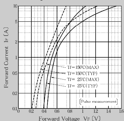
Forward Voltage
