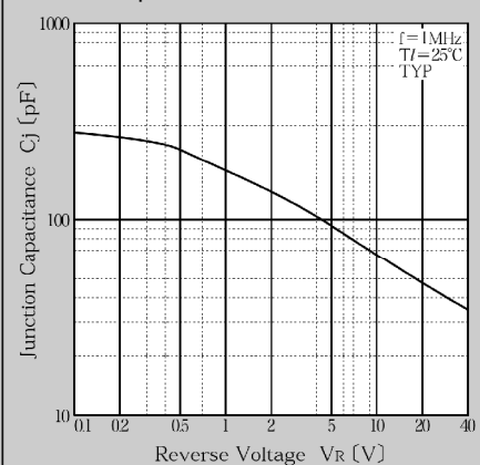
Junction Capacitance
