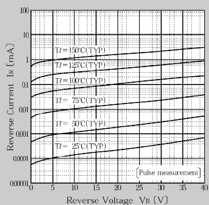
Reverse Current
