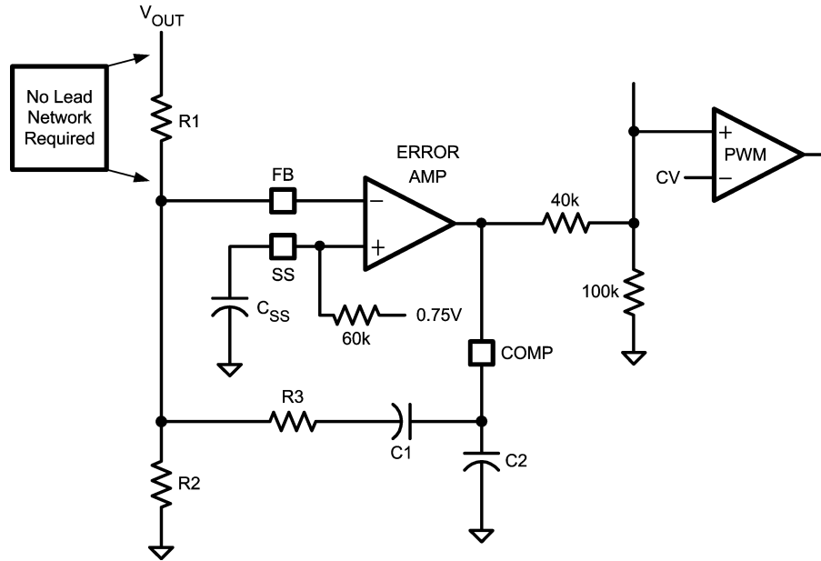
FIGURE 7. Voltage Sensing and Feedback
