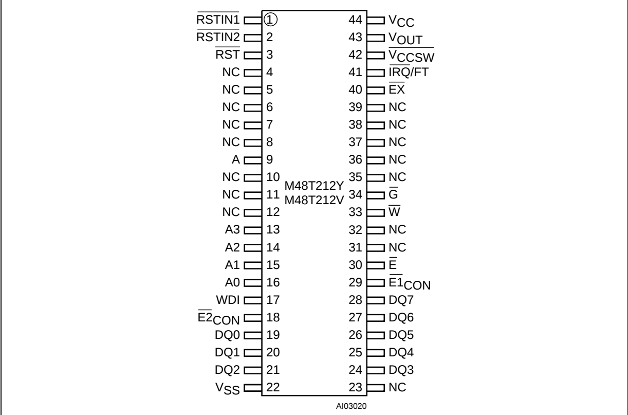
Figure 3. SOIC Connections
