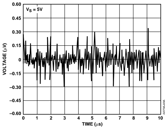
Figure 39. 0.1 Hz to 10 Hz Noise
