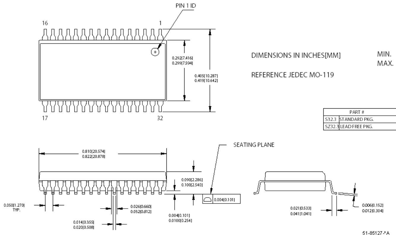
Figure 18. 32-Pin SOIC (51-85127)
