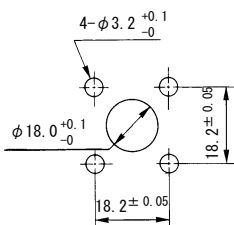
Mounting Hole
