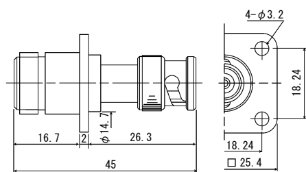
Mounting Hole
