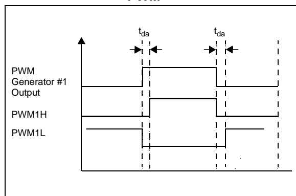
FIGURE 12-15: DEAD-TIME INSERTION FOR COMPLEMENTARY PWM
