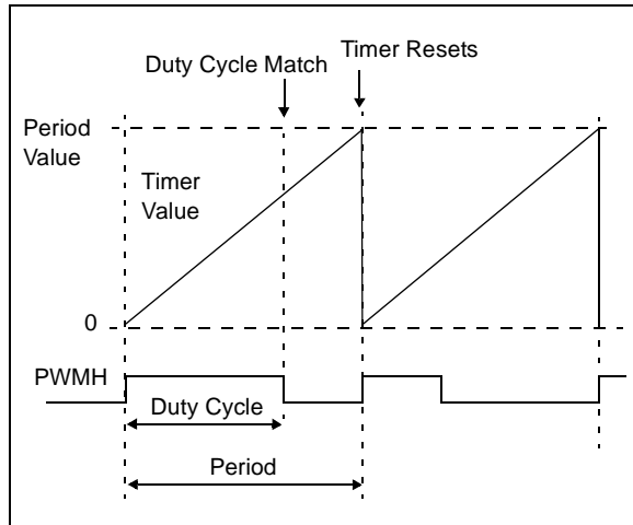
FIGURE 12-3: EDGE-ALIGNED PWM
