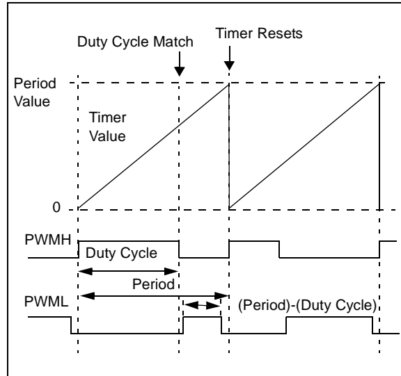
FIGURE 12-4: COMPLEMENTARY PWM
