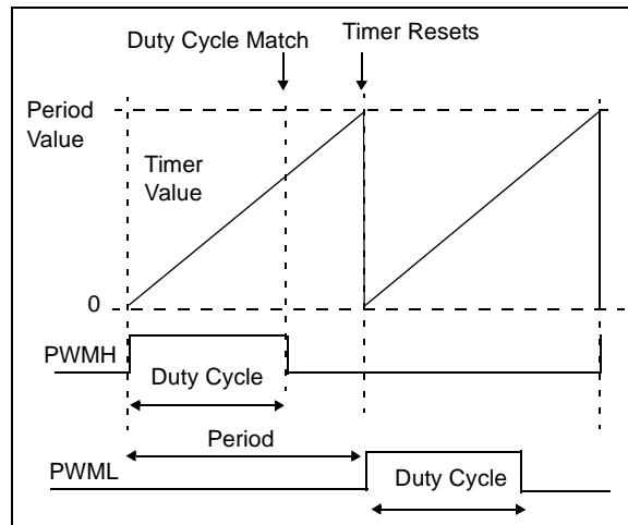
FIGURE 12-5: PUSH-PULL PWM
