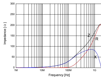
SHB-1S1005-300J
