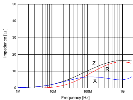
SHB-1T1005-100J
