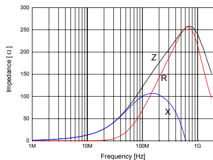
SHB-1M1005-121J
