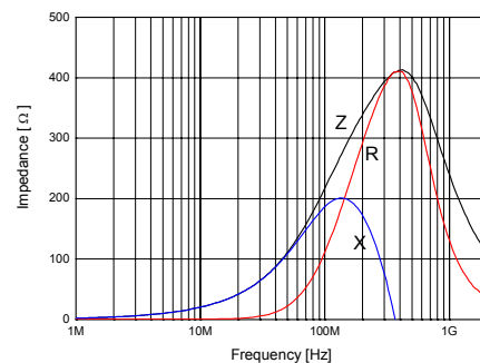
SHB-1M1005-221J
