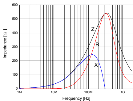
SHB-1M1005-301J
