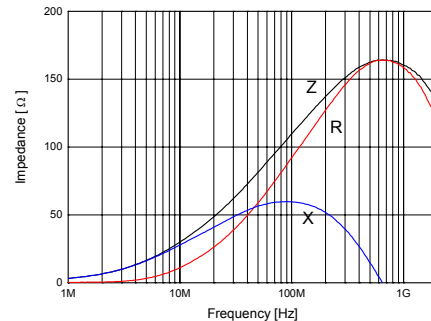
SHB-1T1005-121J
