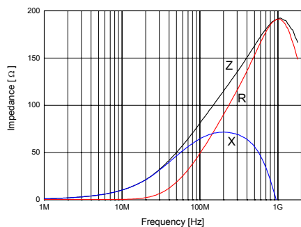
SHB-1M1005-800J
