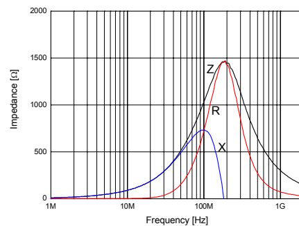
SHB-1M1005-102J
