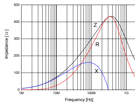
SHB-1T1005-301J
