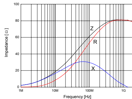
SHB-1T1005-600J
