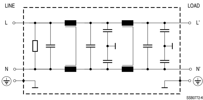
Typical circuit diagram
