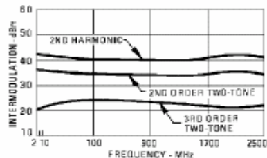
Intermodulation
