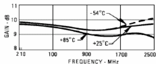
Gain
