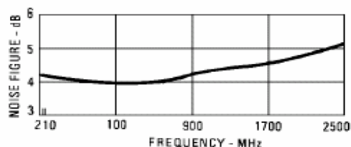
Noise Figure
