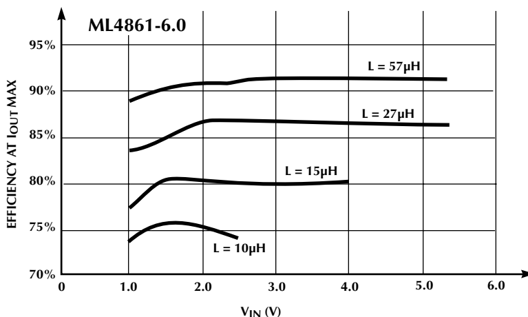
Figure 5. Typical Efficiency as a Function of V_{IN} .
