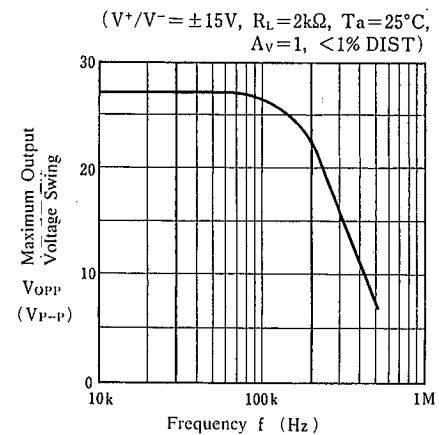
Maximum Output Voltage Swing vs. Frequency
