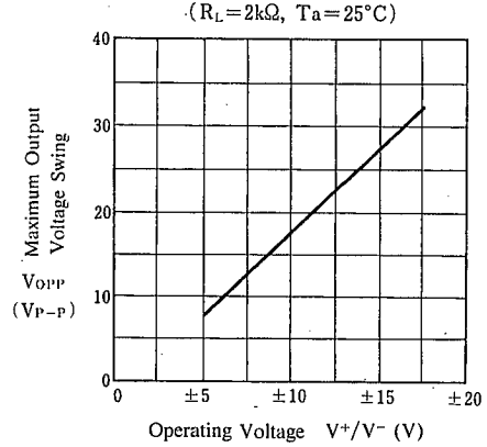
Maximum Output Voltage Swing vs. Operating Voltage
