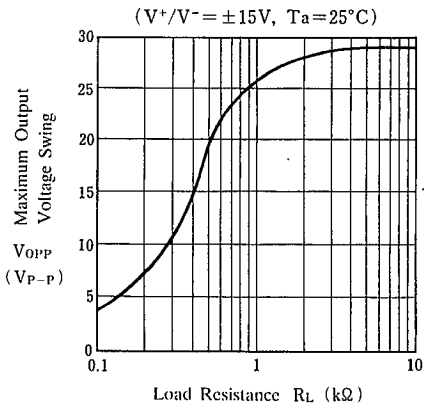
Maximum Output Voltage Swing vs. Load Resistance
