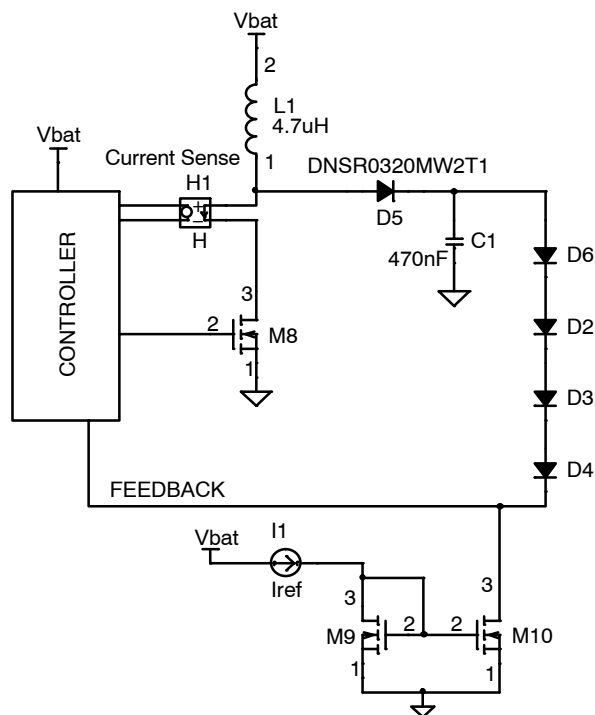
Figure 3. Basic Boost Structure
