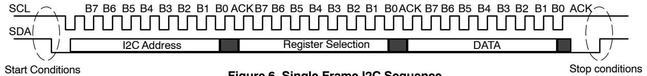
Figure 6. Single Frame I2C Sequence
