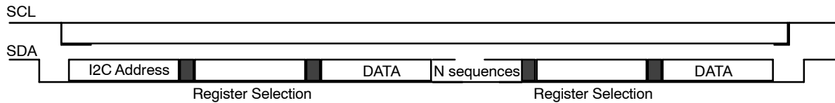
Figure 7. Multi Frames I2C Sequence
