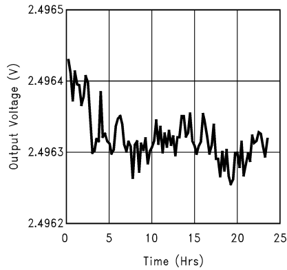
Long Term Drift
