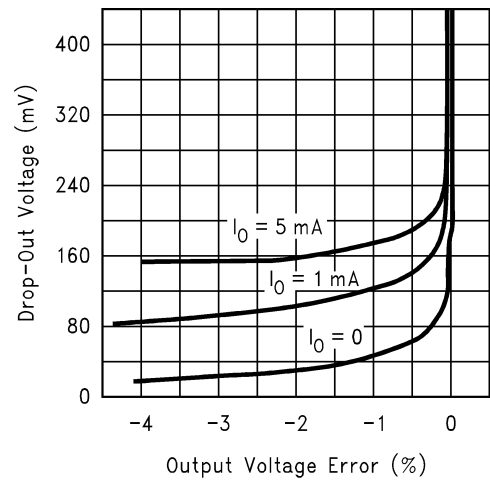
Dropout Voltage vs Output Error
