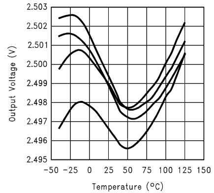
Typical Temperature Drift
