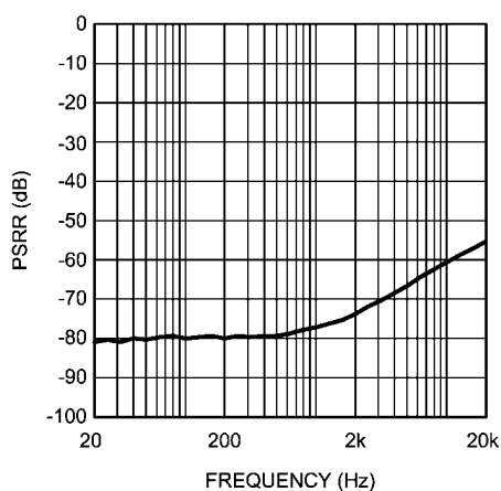
PSRR vs Frequency V_{DD} = 3.6V , R_L = 32\Omega V_{RIPPLE} = 200mV_{PP}
