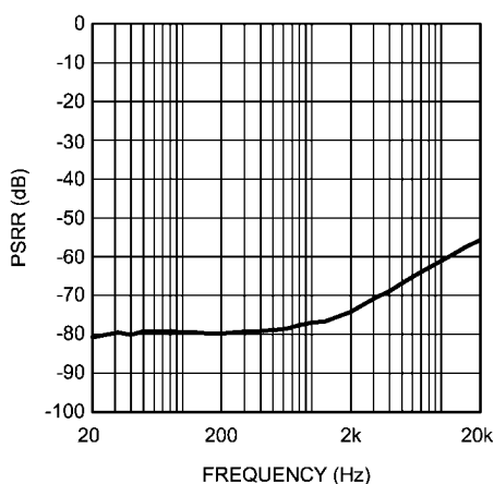
PSRR vs Frequency V_{DD} = 4.2V , R_L = 16\Omega V_{RIPPLE} = 200mV_{PP}
