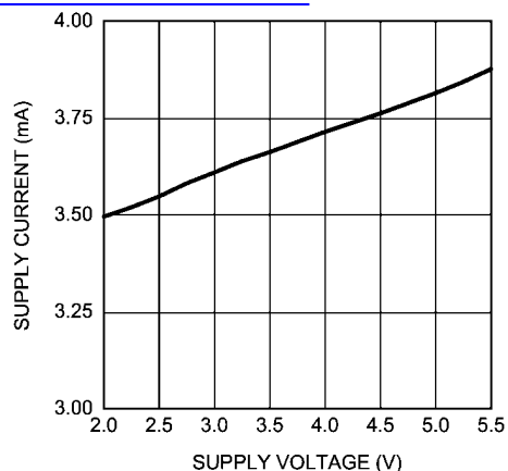
Supply Current vs Supply Voltage V_{IN} = 5V , R_L = 16\Omega 查询"LM48860"供应商
