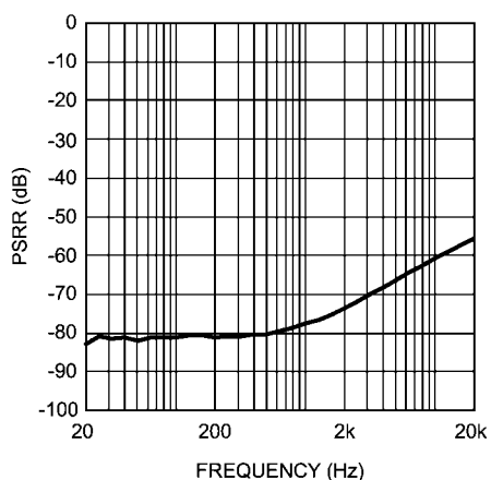
PSRR vs Frequency V_{DD} = 3V , R_L = 16\Omega V_{RIPPLE} = 200mV_{PP}
