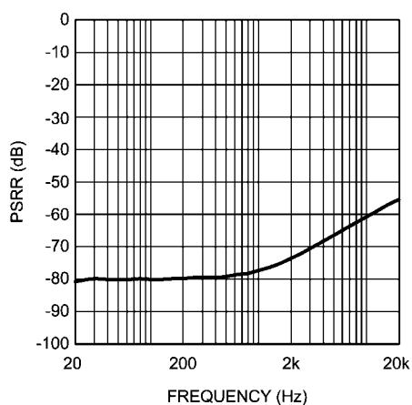
PSRR vs Frequency V_{DD} = 3.6V , R_L = 16\Omega V_{RIPPLE} = 200mV_{PP}
