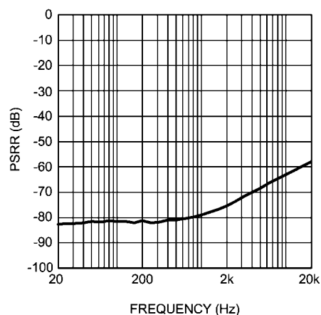
PSRR vs Frequency V_{DD} = 3V , R_L = 32\Omega V_{RIPPLE} = 200mV_{PP}
