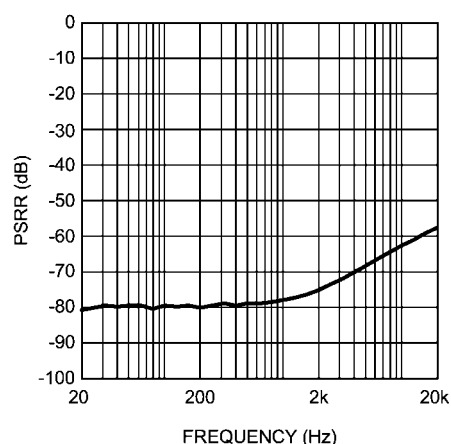
PSRR vs Frequency V_{DD} = 4.2V , R_L = 32\Omega V_{RIPPLE} = 200mV_{PP}
