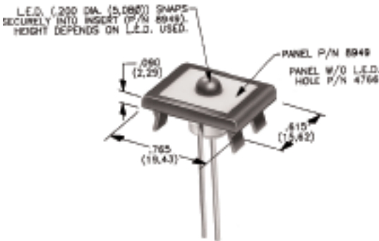
Panel Inserts
