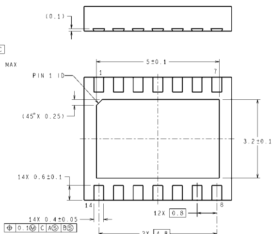
14-Lead LLP Package NS Package Number SRC14A
