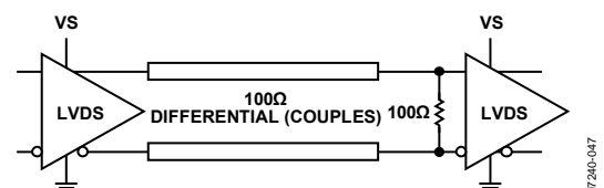
Figure 58. LVDS Output Termination
