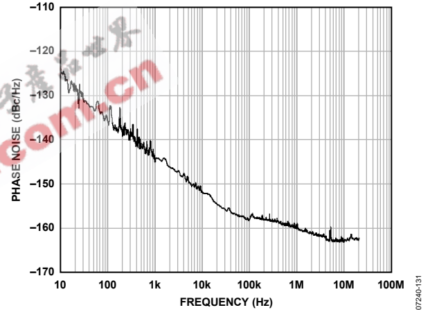
Figure 22. Additive (Residual) Phase Noise, CLK-to-CMOS @ 50 MHz, Divide-by-20
