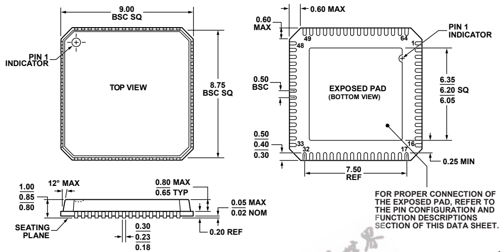
Figure 61. 64-Lead Lead Frame Chip Scale Package (LFCSP_VQ)
