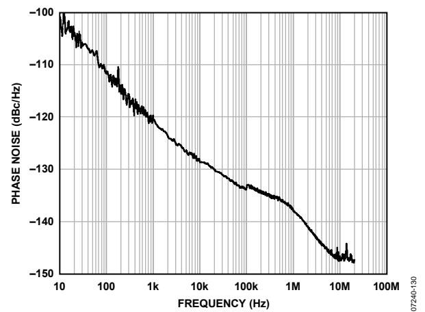
Figure 21. Additive (Residual) Phase Noise, CLK-to-LVDS @ 800 MHz, Divide-by-1
