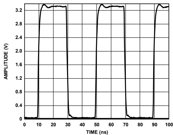
Figure 15. CMOS Output with 10 pF Load @ 25 MHz
