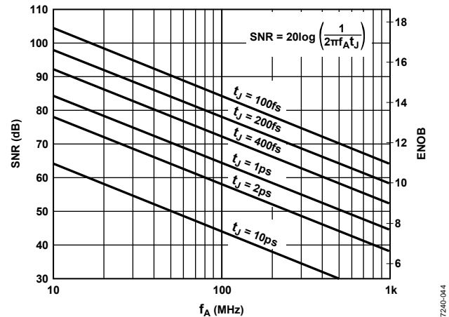
Figure 57. SNR and ENOB vs. Analog Input Frequency
