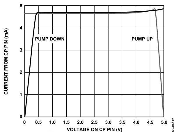
Figure 9. Charge Pump Characteristics @ V_{CP} = 5.0\text{ V}
