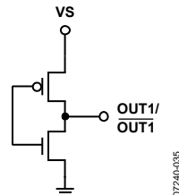
Figure 42. CMOS Equivalent Output Circuit
