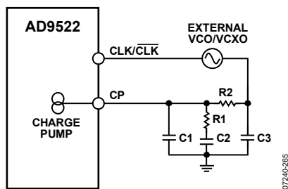
Figure 29. Example of External Loop Filter for PLL
