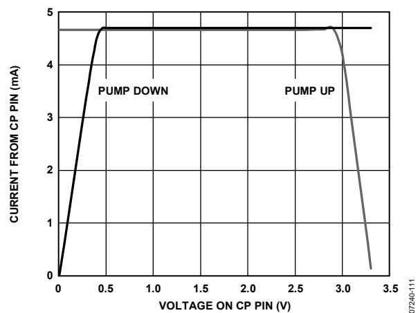
Figure 8. Charge Pump Characteristics @ V_{CP} = 3.3\text{ V}
