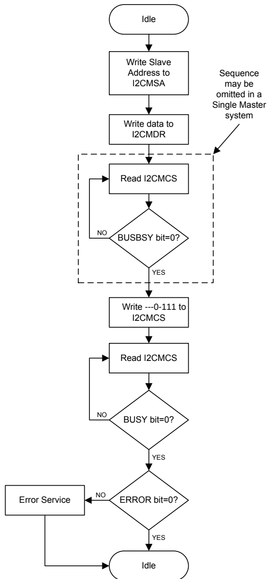
Figure 14-7. Master Single SEND
