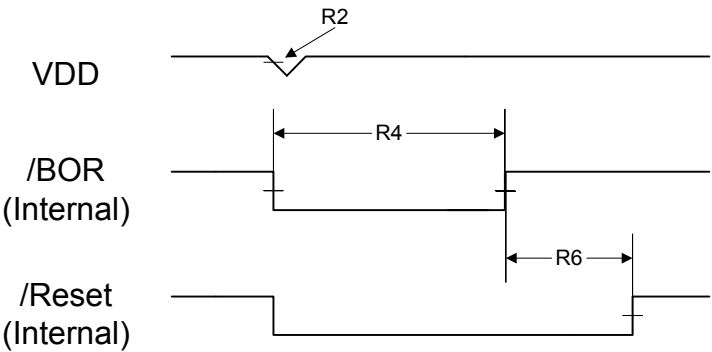
Figure 21-13. Software Reset Timing
