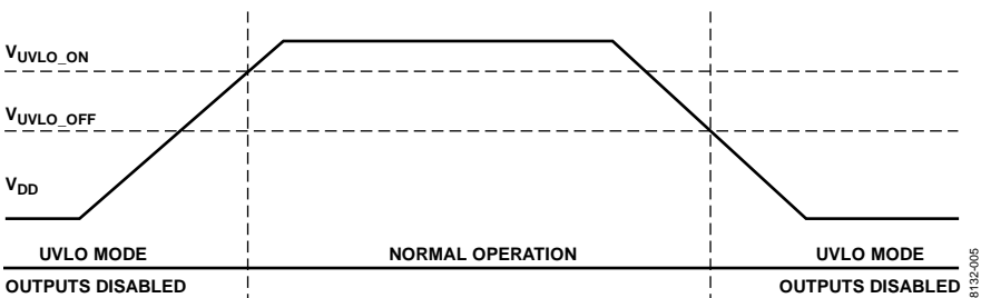
Figure 5. UVLO Function
