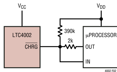
Figure 1. Microprocessor Interface
