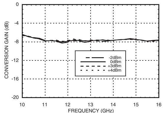
Upconverter USB, IF= 3 GHz Conversion Gain vs. LO Drive
