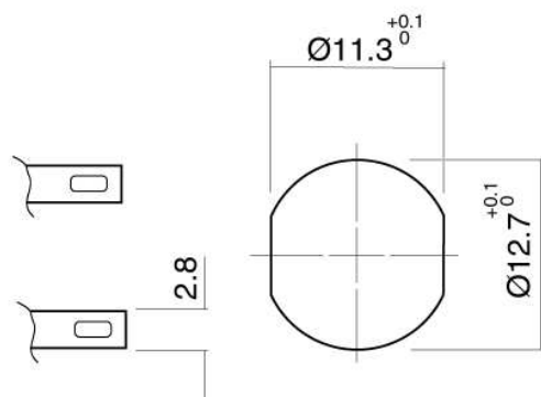
MOUNTING HOLE
