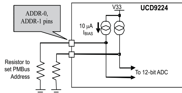
Figure 6. PMBus Address Detection Method
