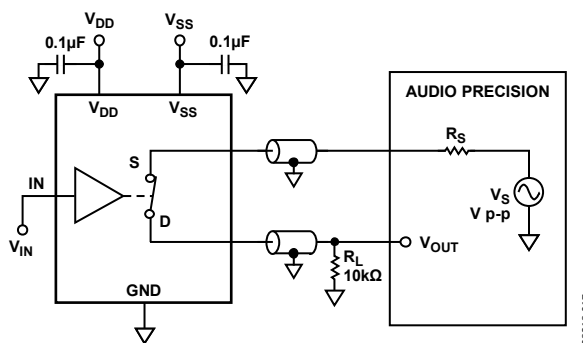
Figure 35. THD + Noise
