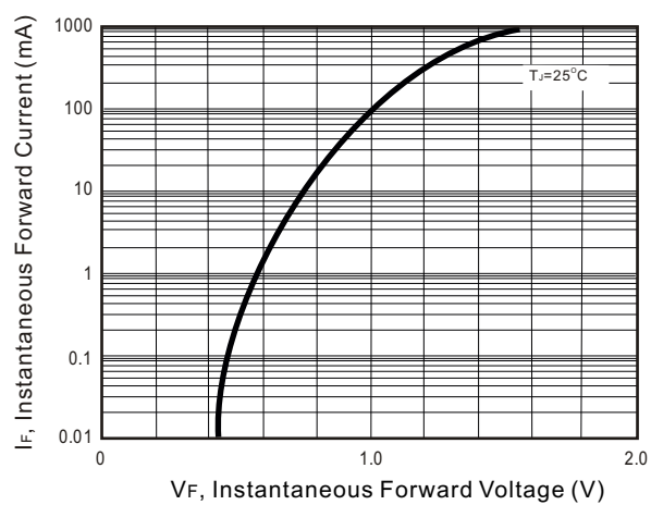
Fig.1 Forward Characteristics
