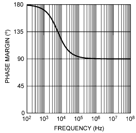
Error Amplifier Phase
