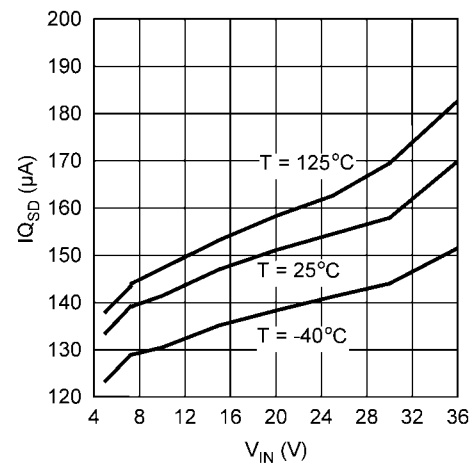
Shutdown I_Q vs. V_{IN}
