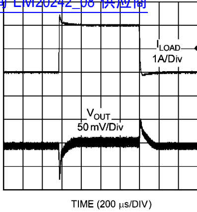
Load Transient Response 查询"LM20242_08"供应商
