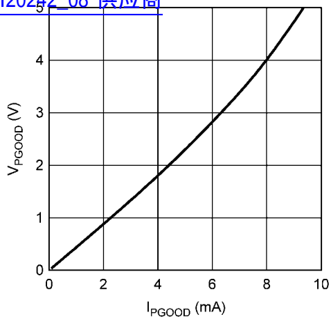
PGOOD V_{OL} vs. I_{PGOOD} 查询"LM20242_08"供应商
