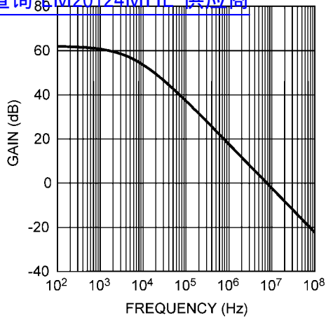
Error Amplifier Gain vs. Frequency 查询"LM20124MHE"供应商
