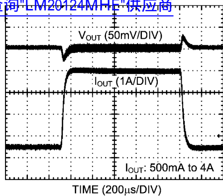
Load Transient Response 查询"LM20124MH-E"供应商
