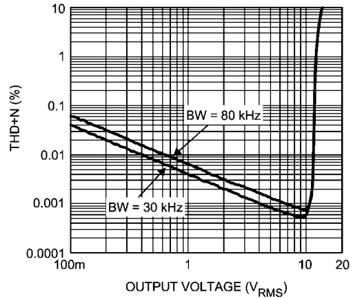
THD+N vs Output Voltage +V_{CC} = -V_{EE} = 20V, f = 1kHz
