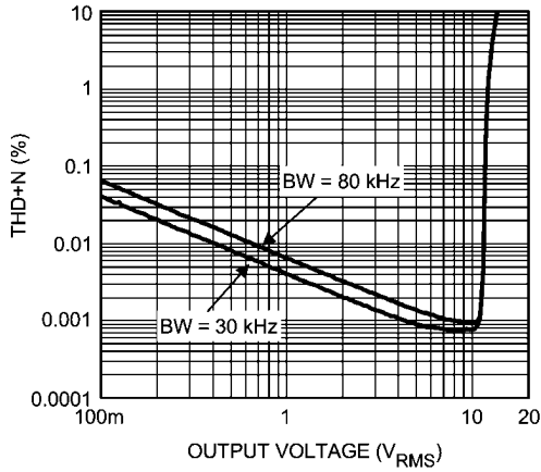
THD+N vs Output Voltage +V_{CC} = -V_{EE} = 20V, f = 20kHz
