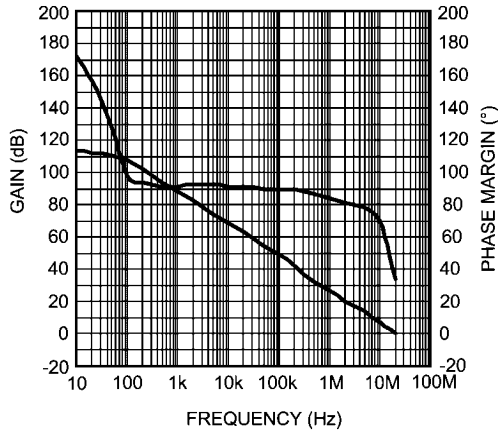
Open Loop Gain and Phase Margin 查询"LME49830"供应商 +V_{CC} = -V_{EE} = 100V
