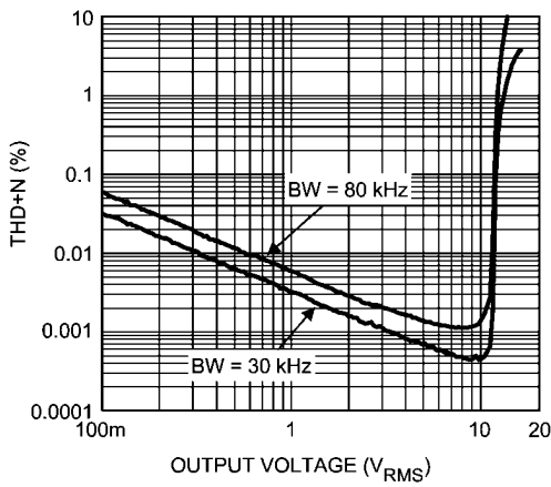
THD+N vs Output Voltage +V_{CC} = -V_{EE} = 20V, f = 20kHz
