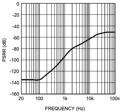
PSRR vs Frequency V_{CC} = +100V , V_{EE} = -100V , No Filters, Input Referred V_{RIPPLE} = 200mV_{RMS} on V_{EE} pin
