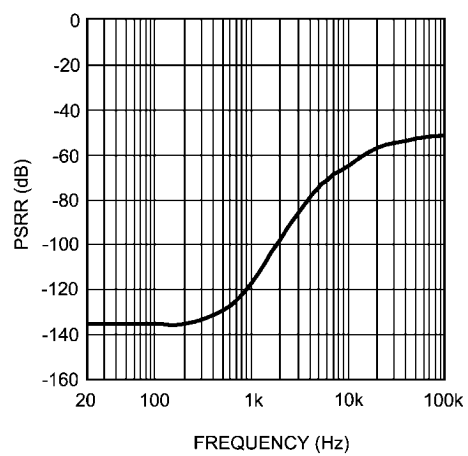
PSRR vs Frequency +V_{CC} = -V_{EE} = 100V, \text{No Filters, Input Referred} V_{RIPPLE} = 200mV_{RMS} \text{ on } V_{CC} \text{ pin}
