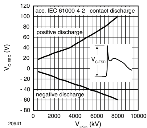
Fig. 9 - Typical Peak Clamping Voltage at \pm ESD Contact Discharge (acc. IEC 61000-4-2)
