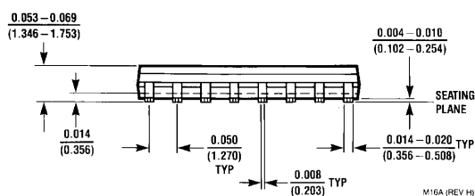
16-Pin SOIC Order Number LMH0024MA NS Package Number M16A
